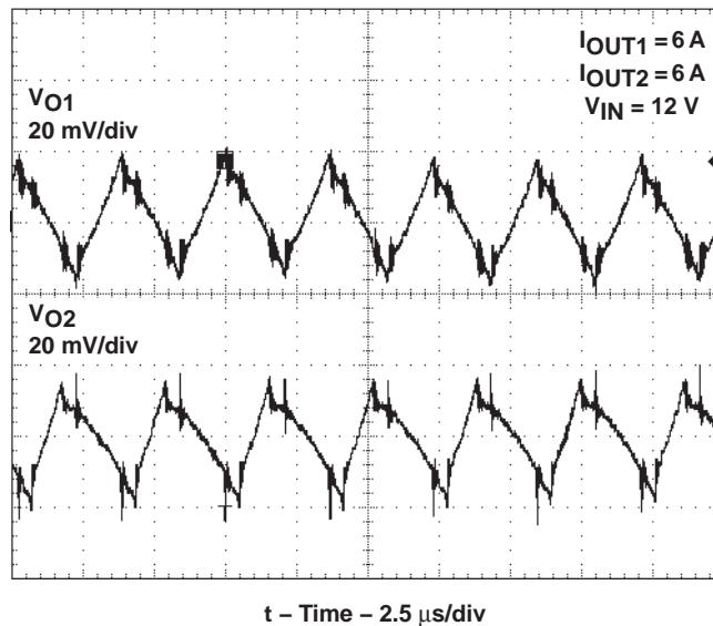
Figure 7. Output Ripple
