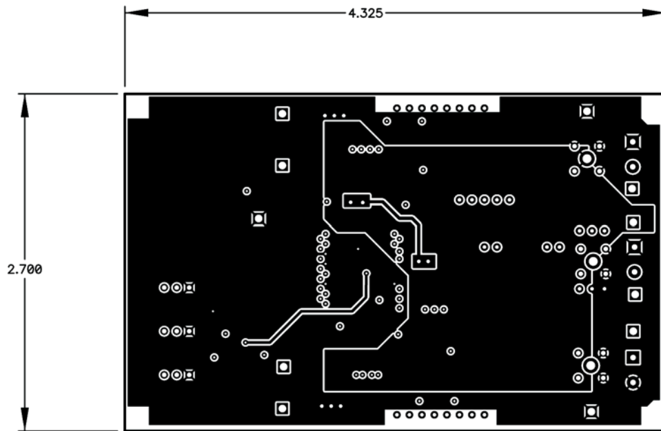
Figure 15. Inner Layer 2
